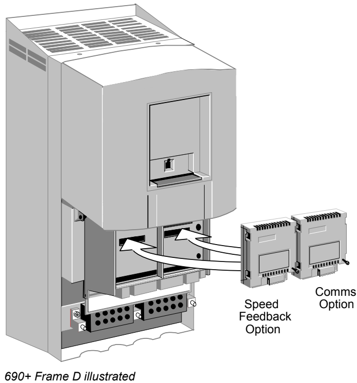
Figure 3. 690+ frames C - J, and 590+ all frame sizes
