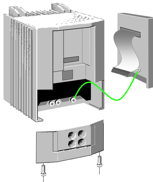
Figure 2. 690+ Frame B
