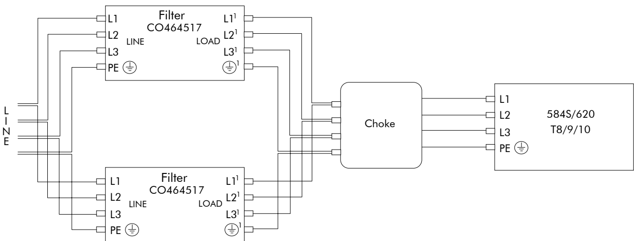
Figure B-5 Using 2 off Part No. CO464517 Type 9 (2200) and Type 10
