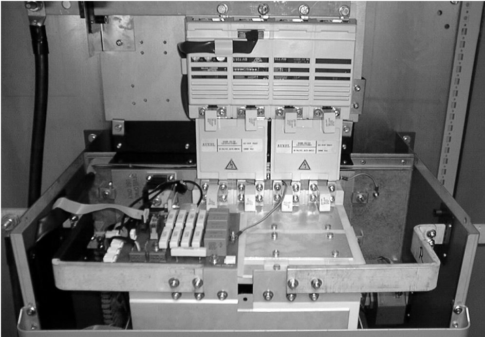
Figure 8-3 Top View of Exhaust Duct/Brake Unit/Inverter Assembly showing the Brake Connecting Plate(s) and Snubber Capacitors fitted
