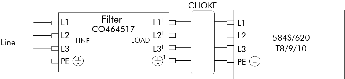
Figure B-3 Wiring Details Using 1 off Part No. CO464517 for Type 8
