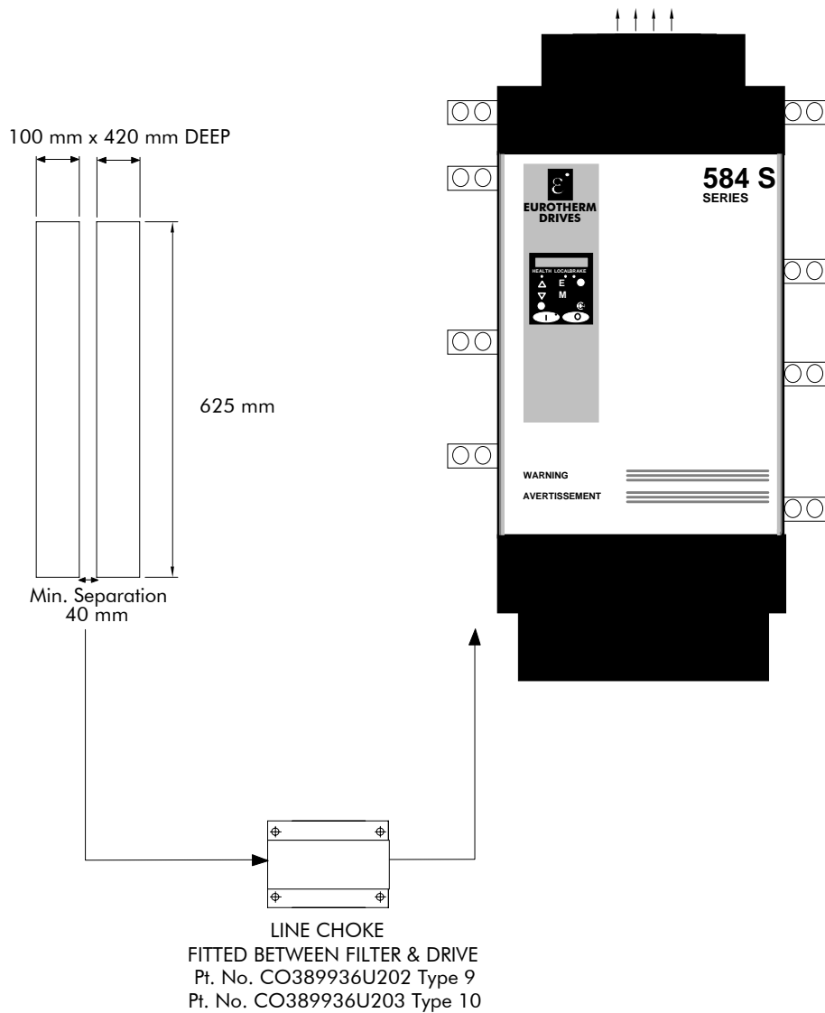
Figure B-5 Using 2 off Part No. CO464517 Type 9 (2200) and Type 10
