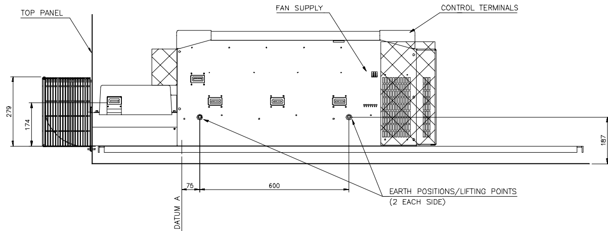
Size 8 Typical Cubicle Installation Outline Drawing (HG 463009 G 003)
