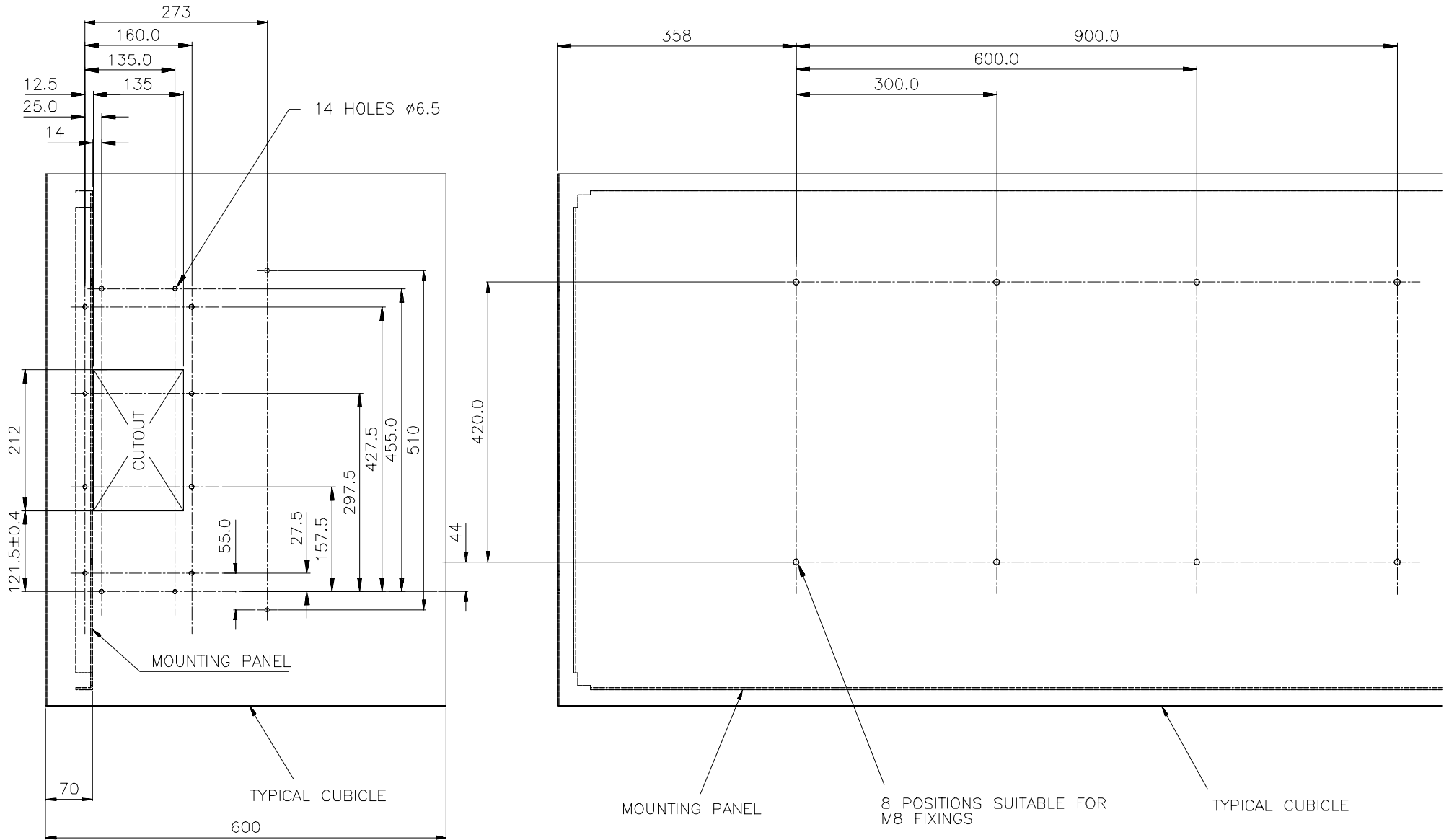
Size 8 Typical Cubicle Machining (HG 463010 G 003)
