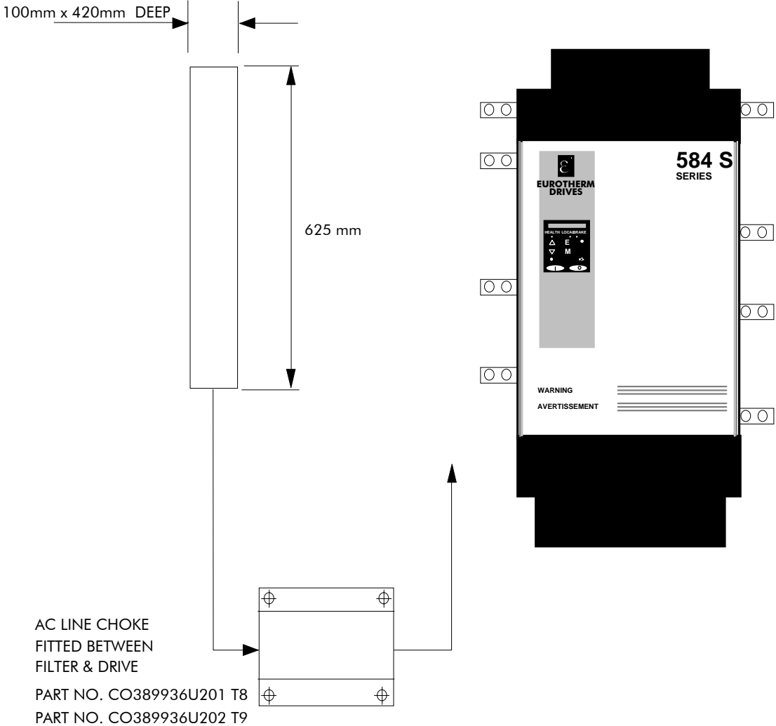
Figure B-2 Filter Mounting Details Using 1 off Part No. CO464517 for Type 8
