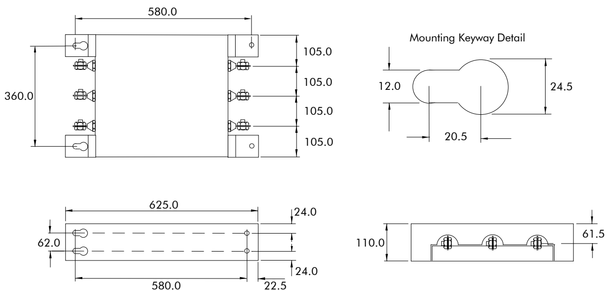
Figure B.1 - AC Supply Filter CO464517D
