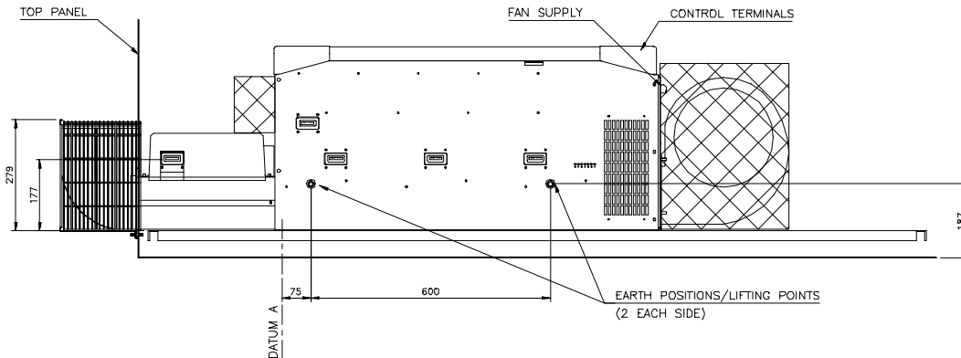
Size 10 Typical Cubicle Installation Outline Drawing (HG 463009 G 001)
