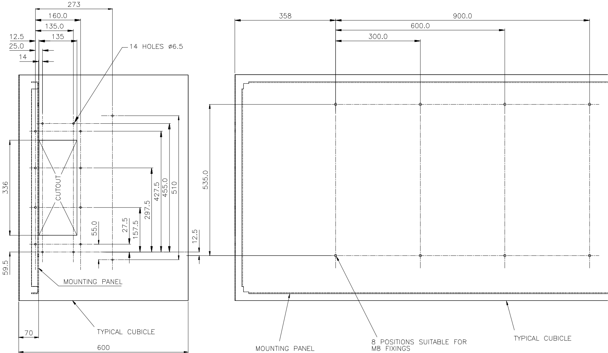
Size 9 Typical Cubicle Machining (HG 463010 G 002)
