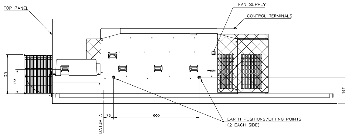
Size 9 Typical Cubicle Installation Outline Drawing (HG 463009 G 002)
