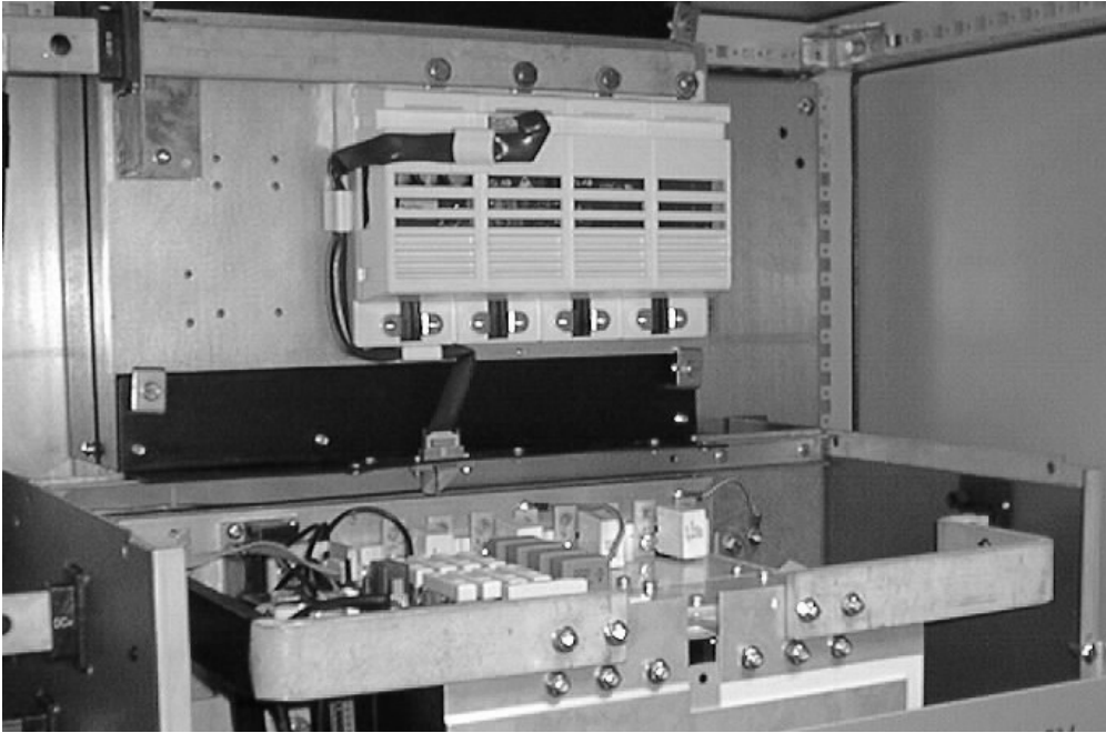
Figure 8-2 View without Brake Connecting Plate(s) showing the Control Cable connection between the Brake Unit and the Inverter
