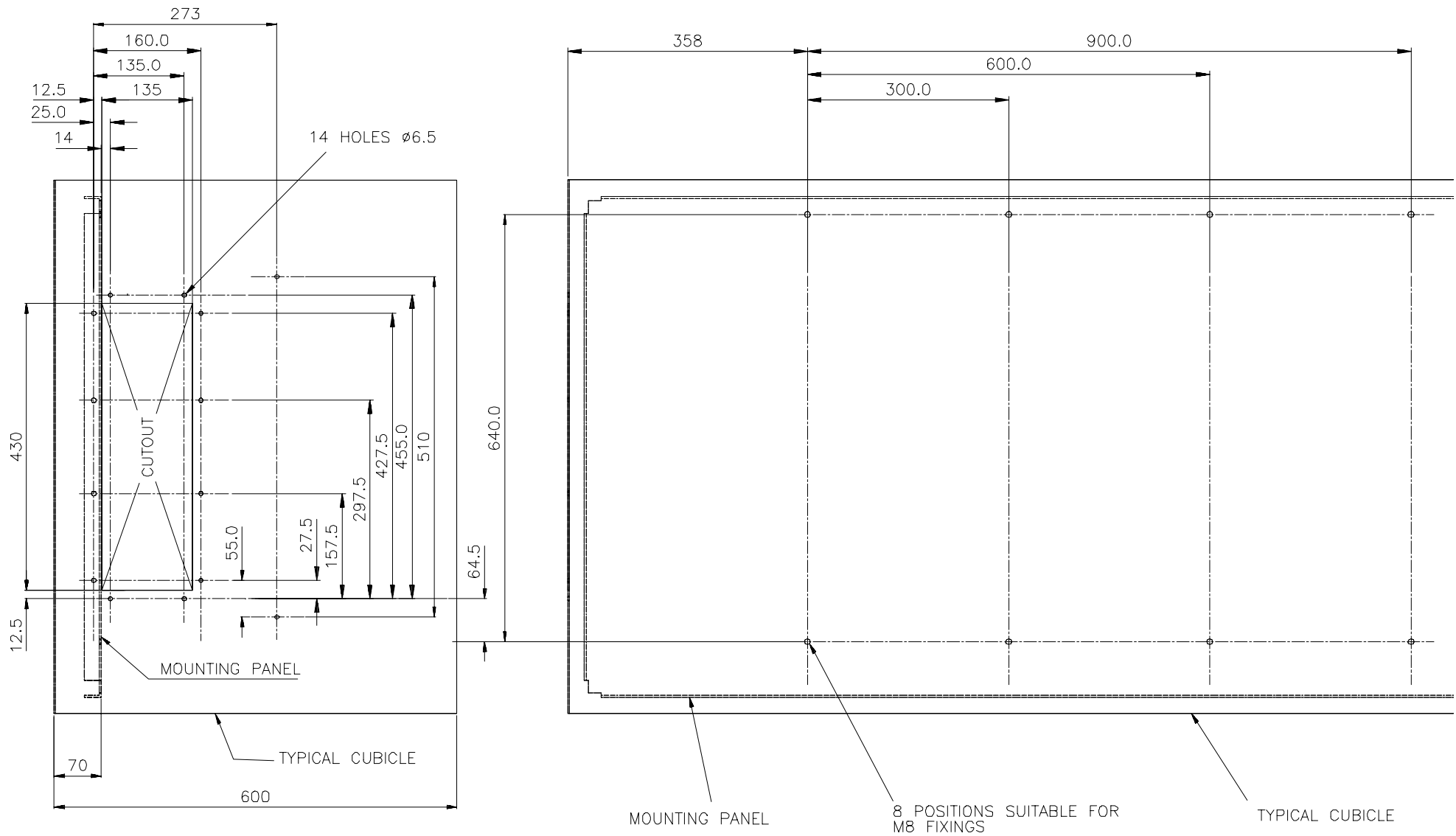
Size 10 Typical Cubicle Machining (HG463010 G 001)
