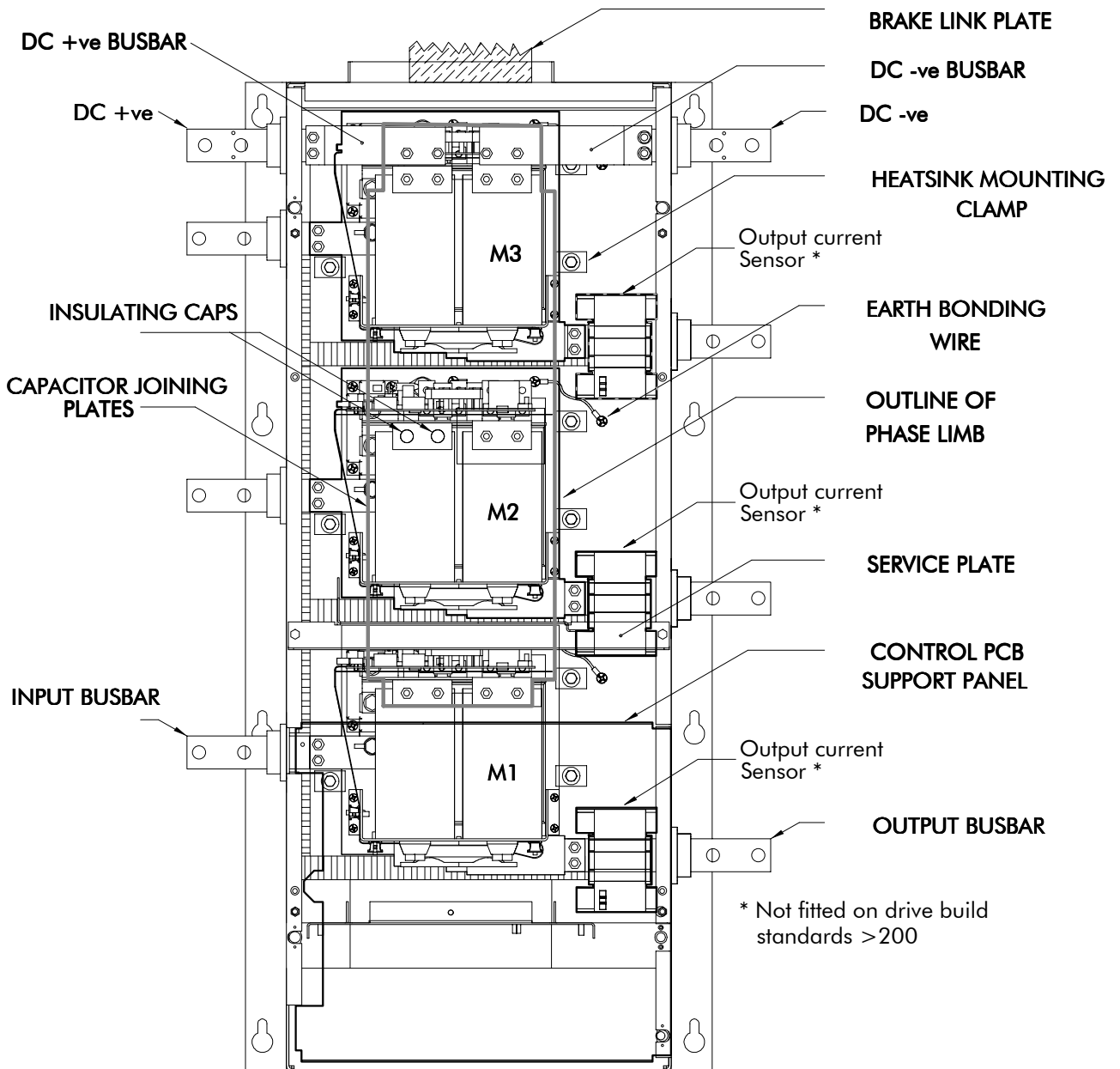
Figure 9.4 Power Component Identification (type 8)
